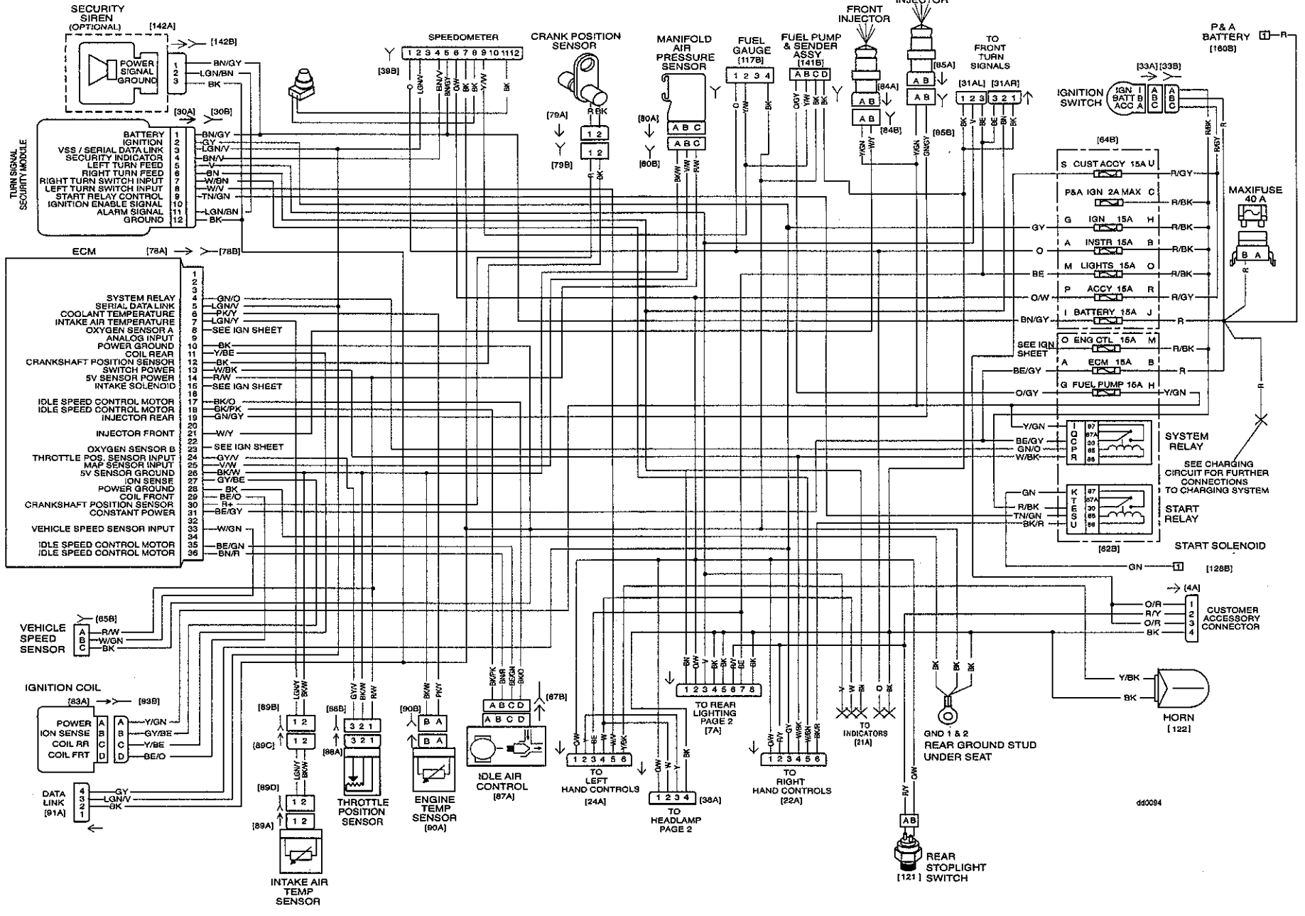
2006 ALL FXDWG, FXD35 DOM. and INT. MODELS, MAIN HARNESS
