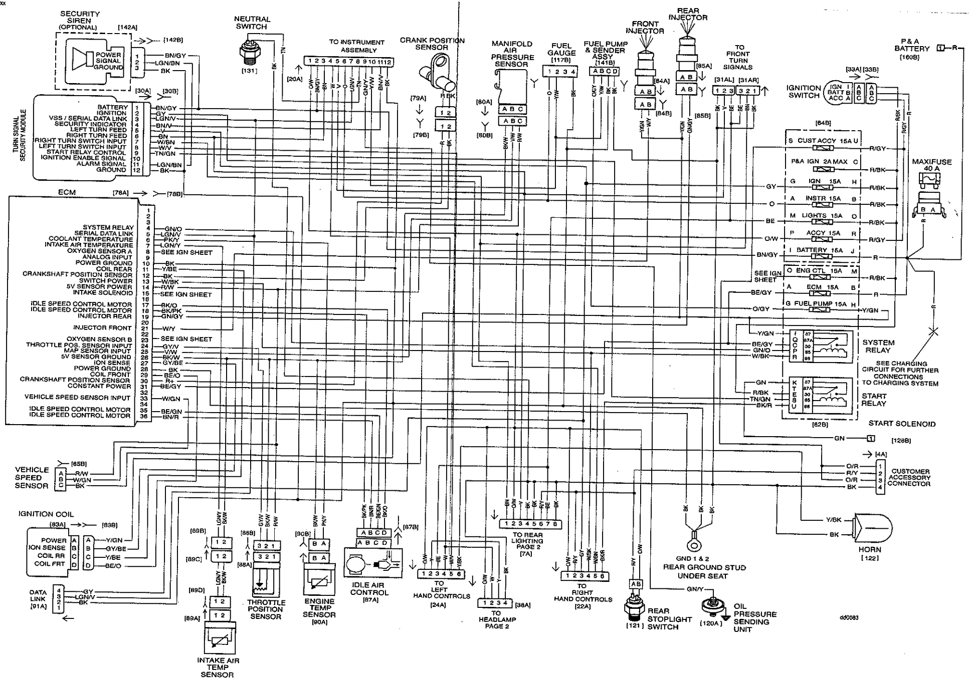
2006 ALL DYNA DOM. and INT. MODELS (Except FXDWG, FXD35), MAIN HARNESS
